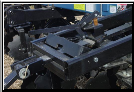
Pull out and swing away wagon hitch
